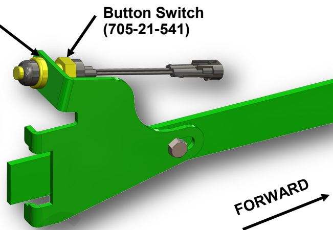
Long Linkage Button Bracket (2755Y1)
